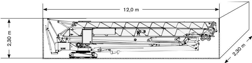
40 ft Open Top Container
