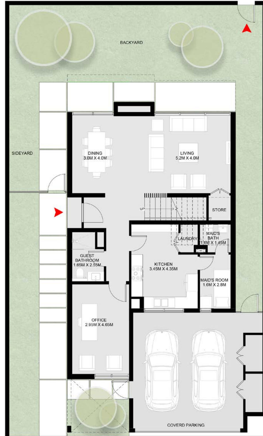
Ground Floor
