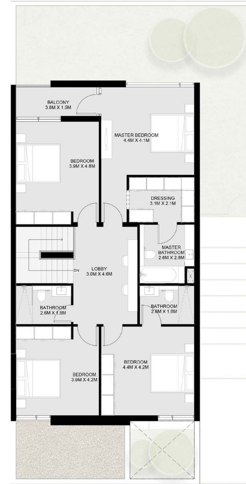
First Floor
