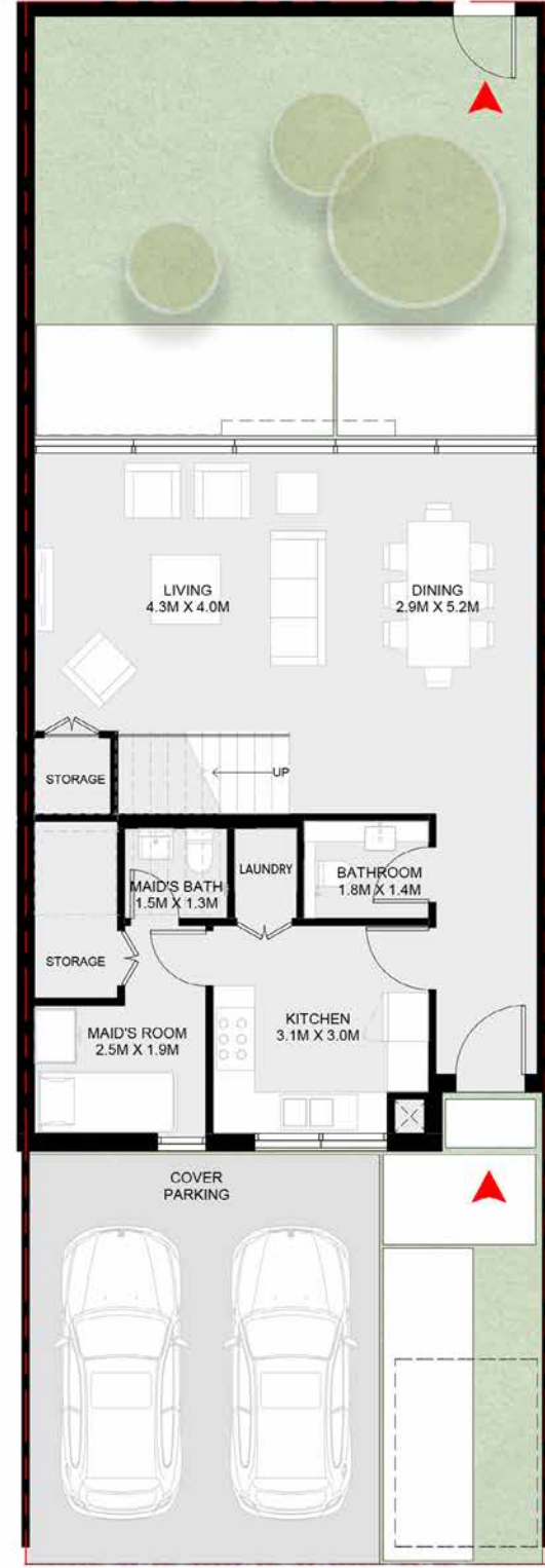
Ground Floor
